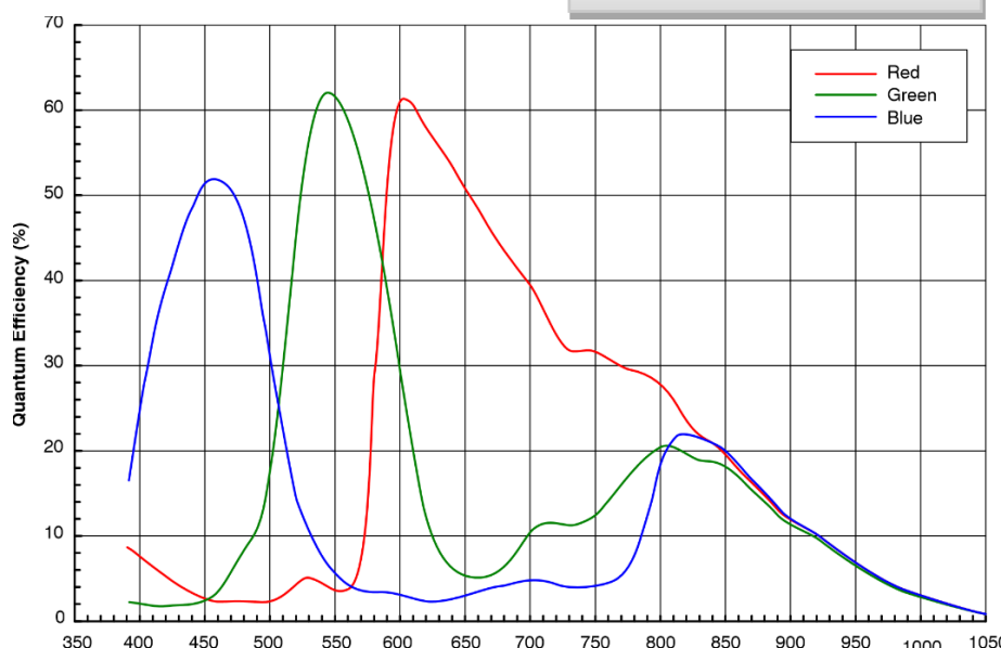
Quantum Efficiency – Color Sensor
