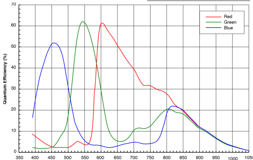
Quantum Efficiency - Color Sensor
