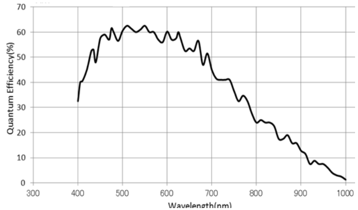
ACH200-NIR Image Sensor Performance
