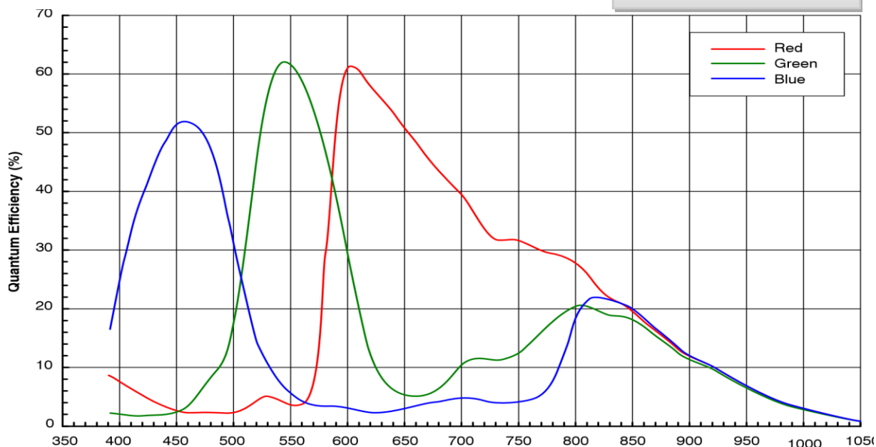
Quantum Efficiency - Color Sensor
